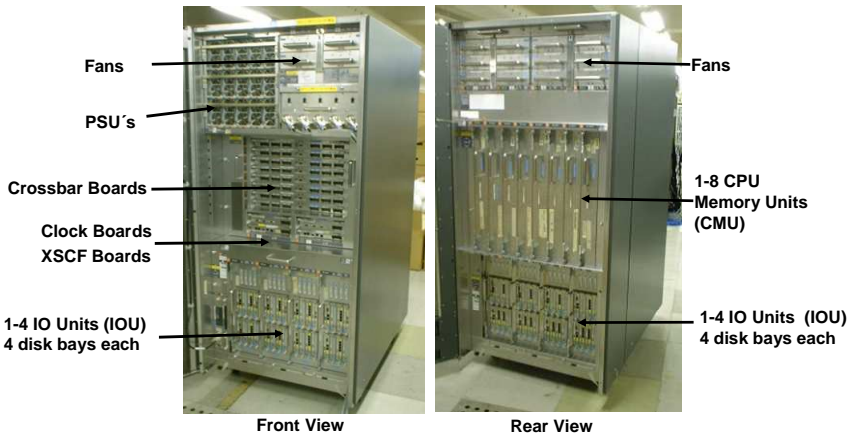
Figure 2-8. Fujitsu Siemens Computers SPARC Enterprise M9000-32 server enclosure diagram..
