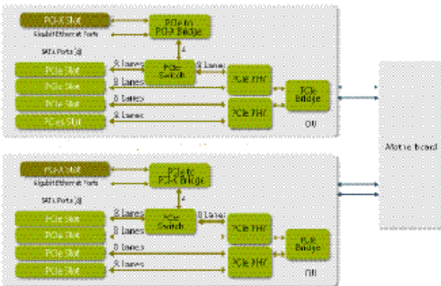
Figure 5-2. Fujitsu Siemens Computers SPARC Enterprise M5000 server I/O subsystem architecture.
