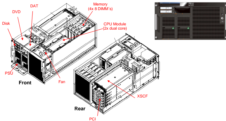
Figure 2-5. Fujitsu Siemens Computers SPARC Enterprise M4000 server enclosure diagram.
