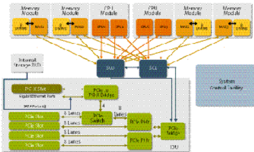
Figure 3-1. Fujitsu Siemens Computers SPARC Enterprise M4000 system interconnect diagram.
