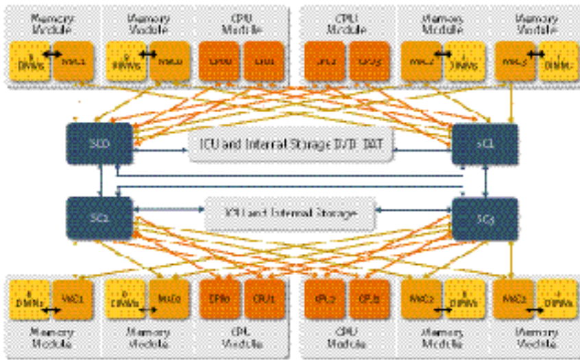
Figure 3-2. Fujitsu Siemens Computers SPARC Enterprise M5000 system interconnect diagram.
