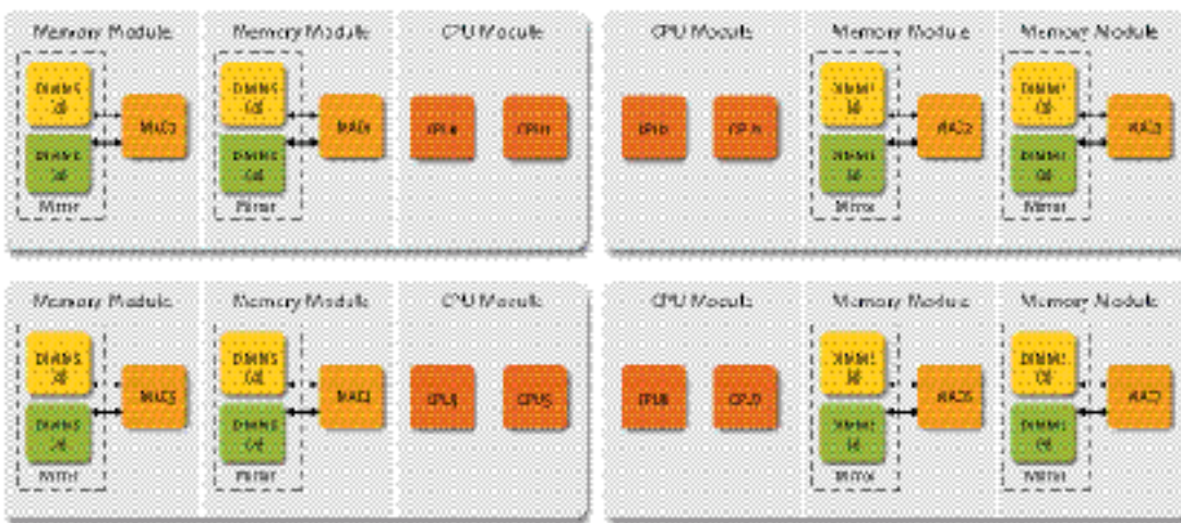
Figure 2-2. Fujitsu Siemens Computers SPARC Enterprise M5000 server memory mirroring architecture.
