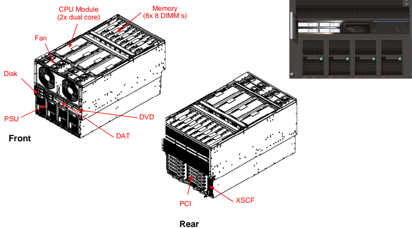
Figure 2-6. Fujitsu Siemens Computers SPARC Enterprise M5000 server enclosure diagram.
