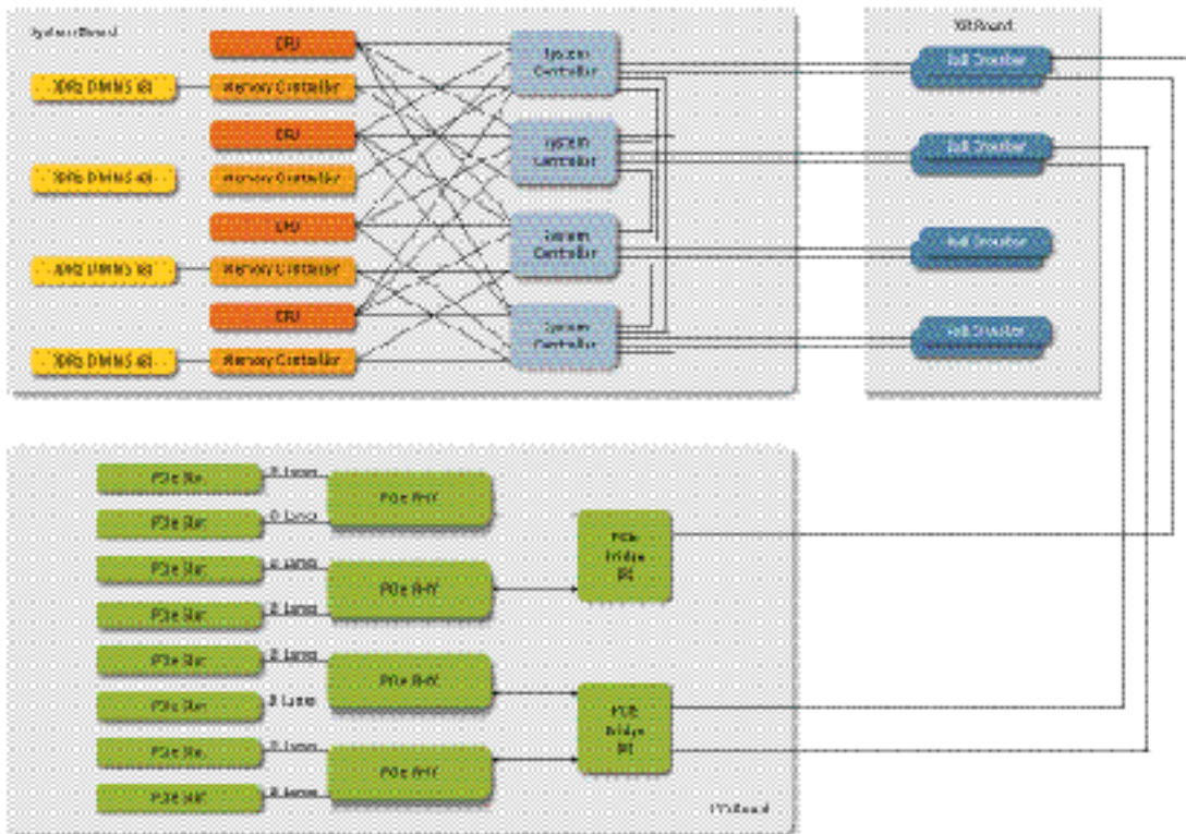
Figure 3-3. Fujitsu Siemens Computers SPARC Enterprise M8000 and Fujitsu Siemens Computers SPARC Enterprise M9000 system interconnect diagram
