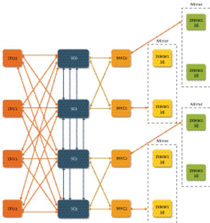
Figure 2-3. Fujitsu Siemens Computers SPARC Enterprise M8000 and Fujitsu Siemens Computers SPARC Enterprise M9000 server memory mirroring architecture.
