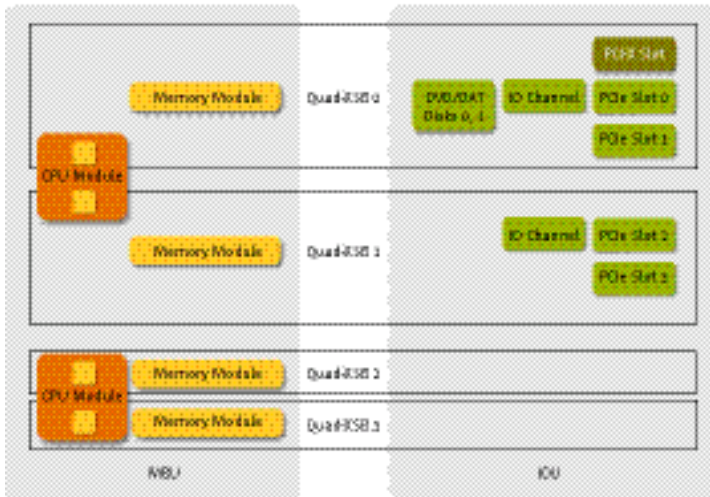
Figure 6-1. Fujitsu Siemens Computers SPARC Enterprise M4000 server Quad-XSB configuration.
