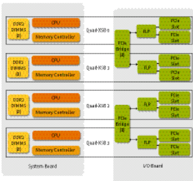
Figure 6-2. Fujitsu Siemens Computers SPARC Enterprise M8000 and Fujitsu Siemens Computers SPARC Enterprise M9000 system board Quad-XSB configuration.
